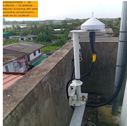
Mobitel Existing GPS antenna
