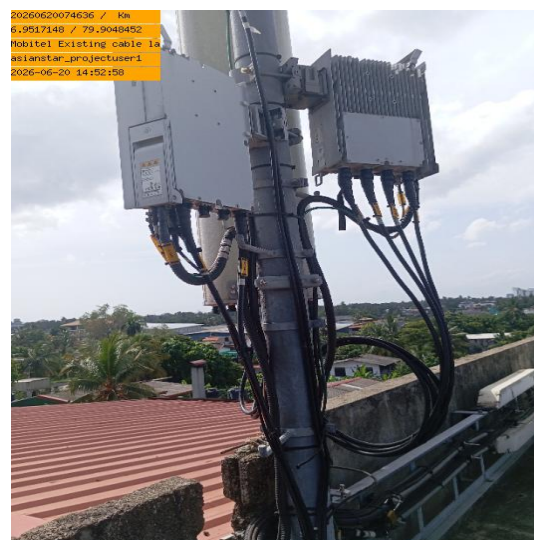
Mobitel Existing cable ladder (Vertical )
